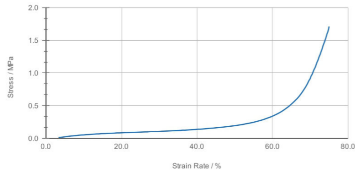
Stress Strain Curve
